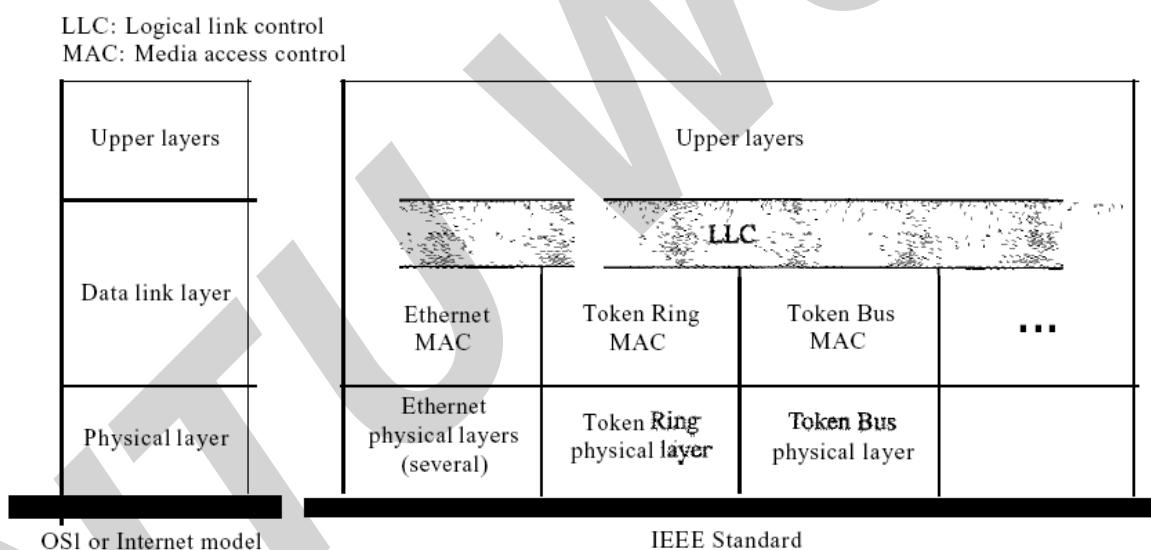
Figure 1 IEEE standard for LANs
