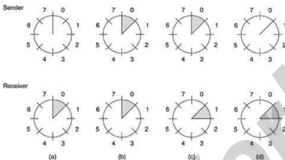
Fig.8. A sliding window of size 1, with a 3-bit sequence number (a) Initially (b) After the first frame has been sent (c) After the first frame has been received (d) After the first acknowledgement has been received.
