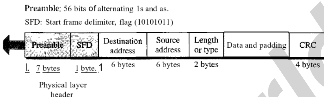
Figure 4 802.3 MAC frame
