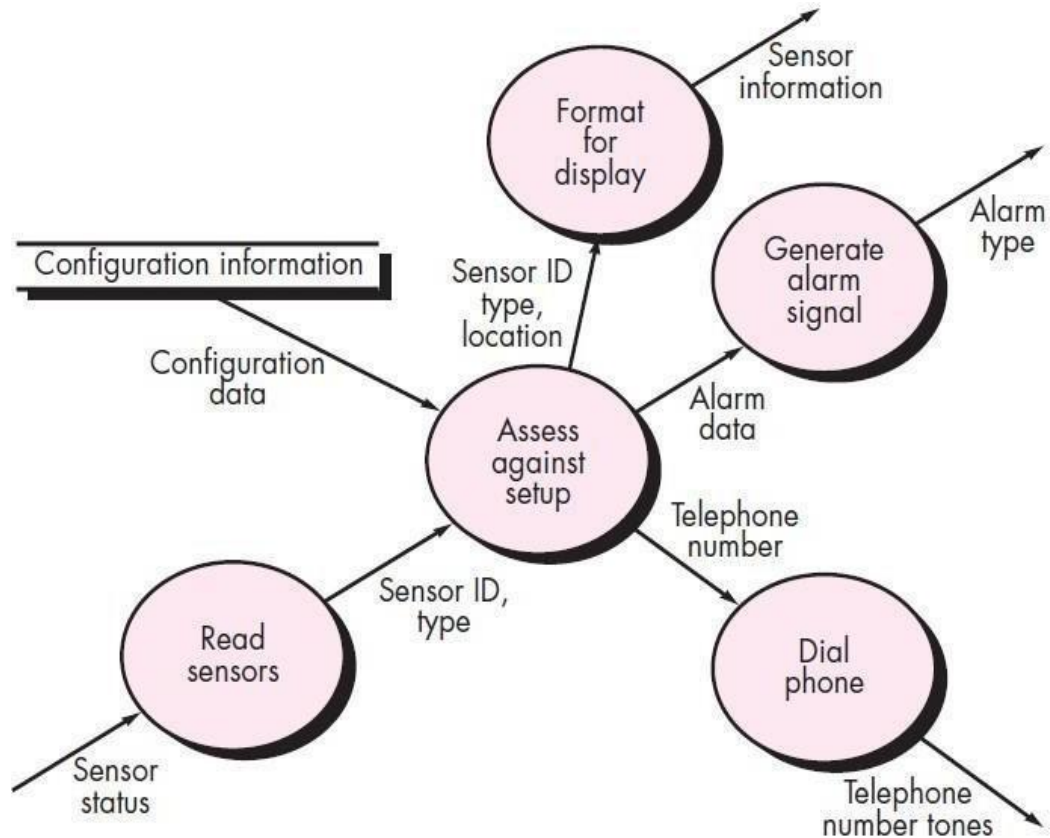
Fig : Level 2 DFD that refines the monitor sensors process
